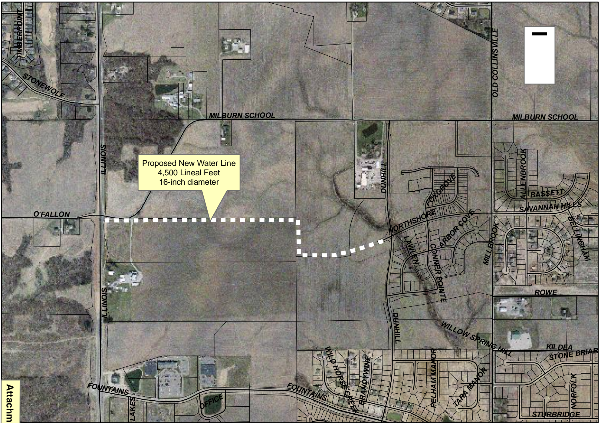
Proposed Water Line from IL-159 to Fountains Subdivision
